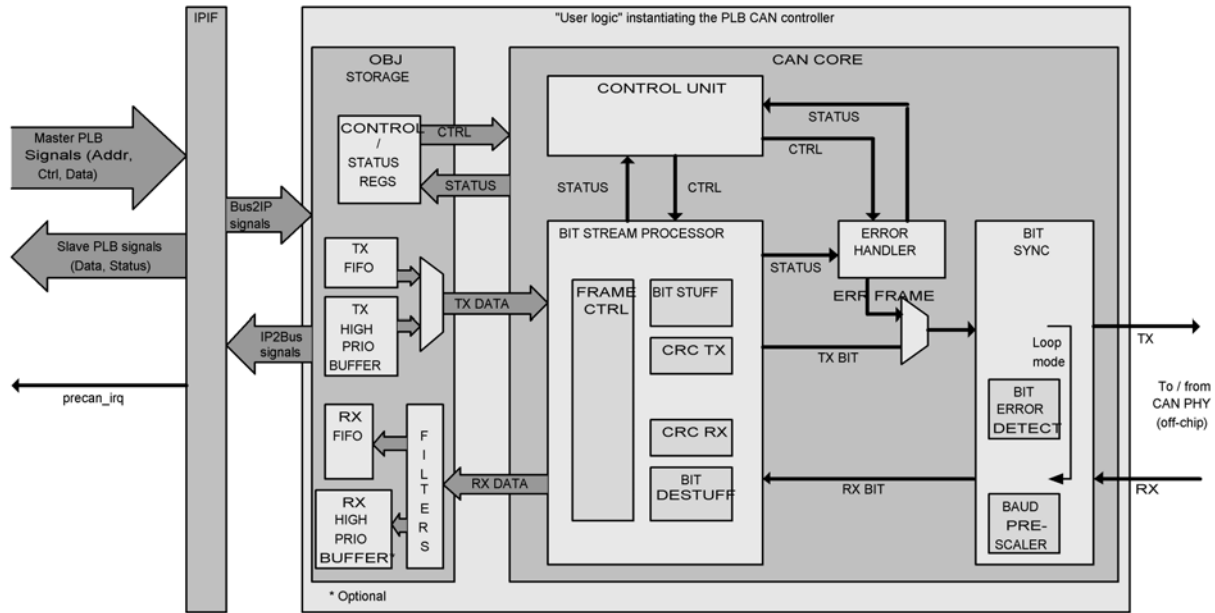
Figure1. CAN Controller IP Block diagram
